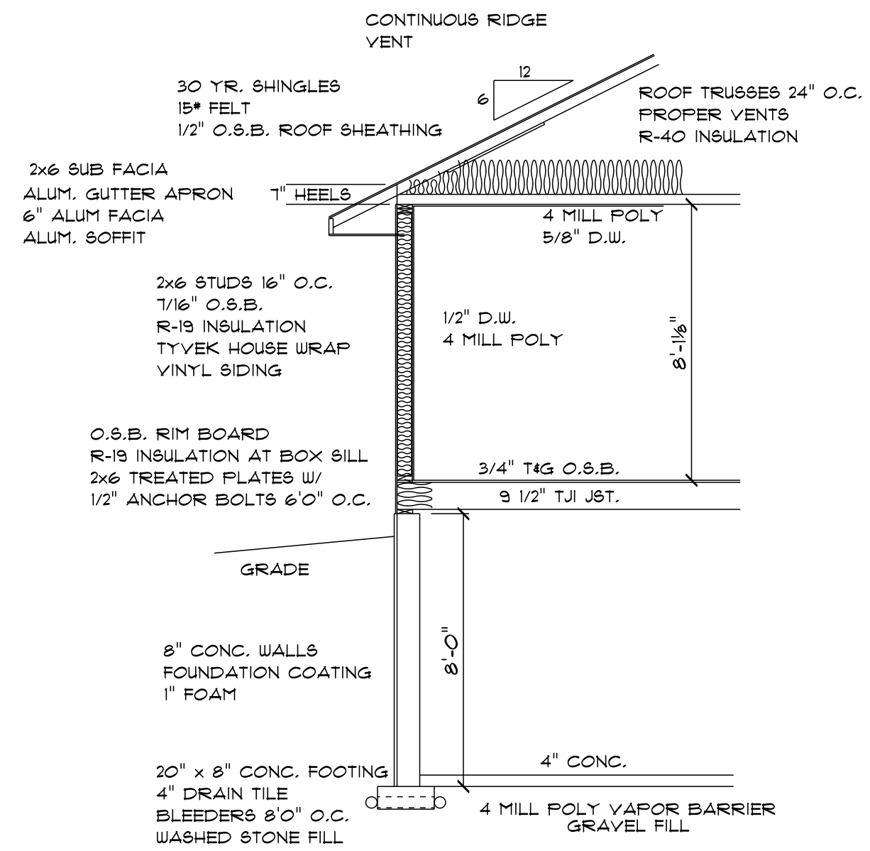
TYPICAL SECTION
