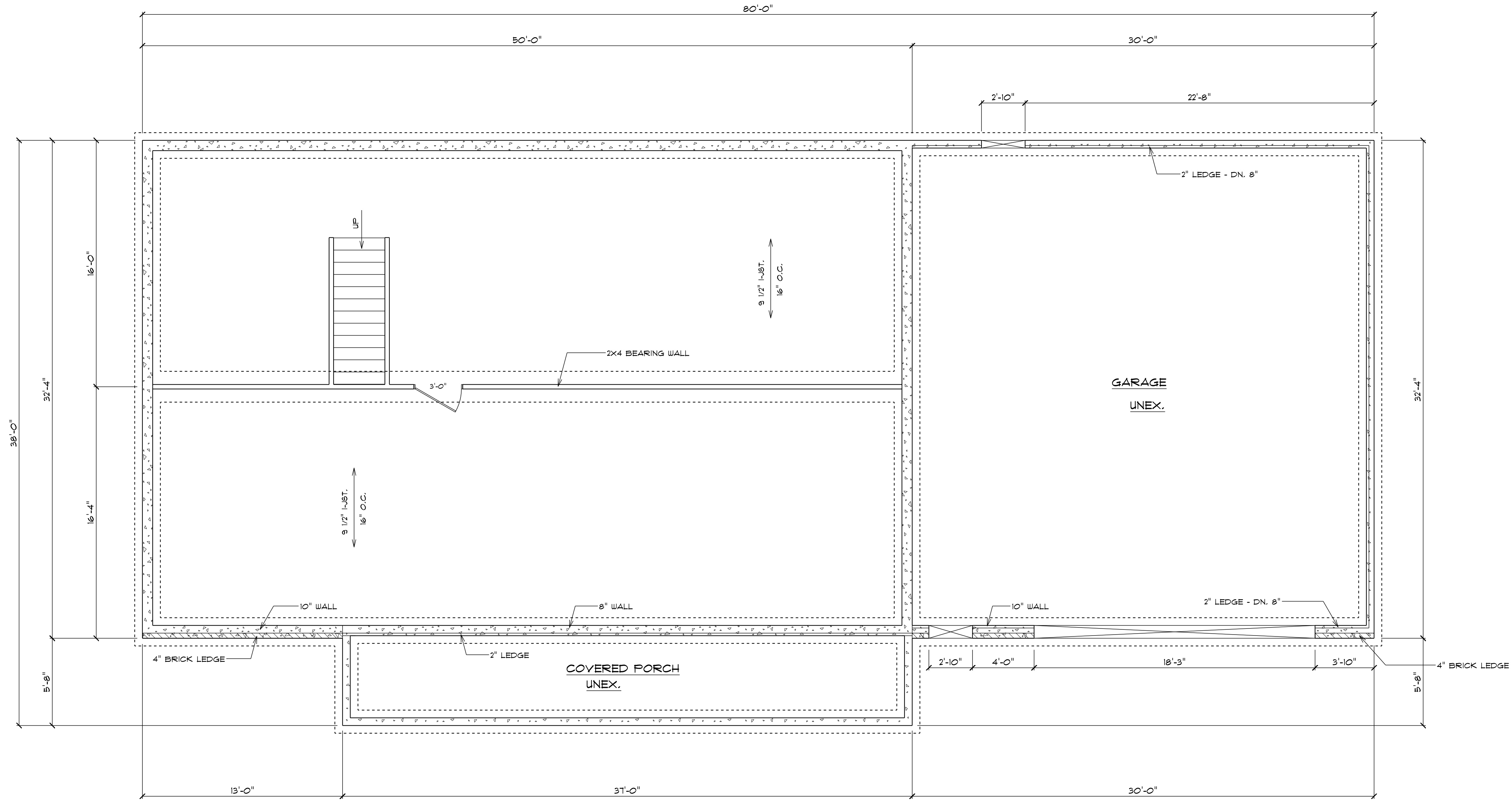
FOUNDATION PLAN 8' HT. WALLS
